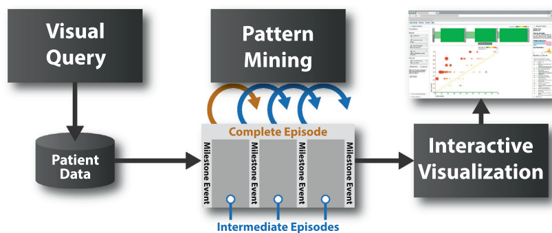
Fig. 1. The visual query component provides an intuitive user interface for authoring episode constraints. Patient data that matches the episode definition is retrieved and passed to the event pattern-mining module. Mining is first performed on the complete episode. The same mining algorithm is then performed on all intermediate episodes. Finally, an interactive visualization lets users explore the results and uncover temporal trends.
