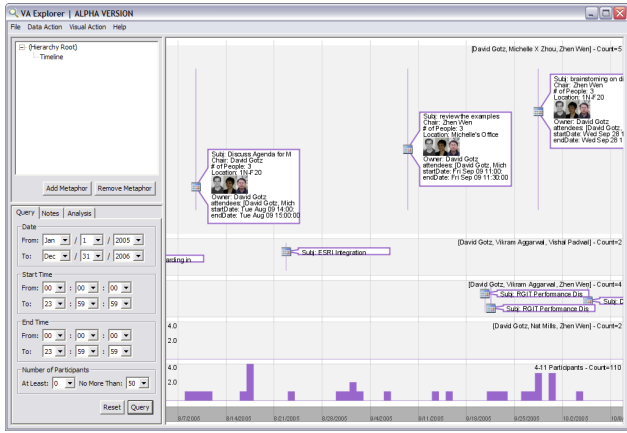
Figure 10: A screen shot from the HARVEST prototype for analyzing organizational communications data in our first case study.
