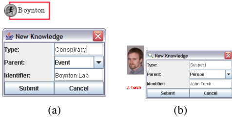
Figure 3: (a) Create is used to define newly synthesized knowledge without direct evidence. (b) Annotation is used when direct evidence is available.
